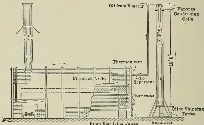
FIG. 104.—Plant for Dehydrating Petroleum.
